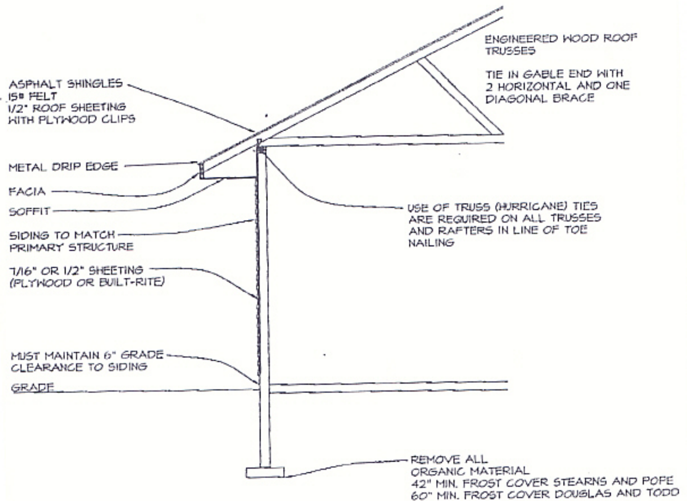
SLAB ON GRADE CONSTRUCTION EXHIBIT (9)
